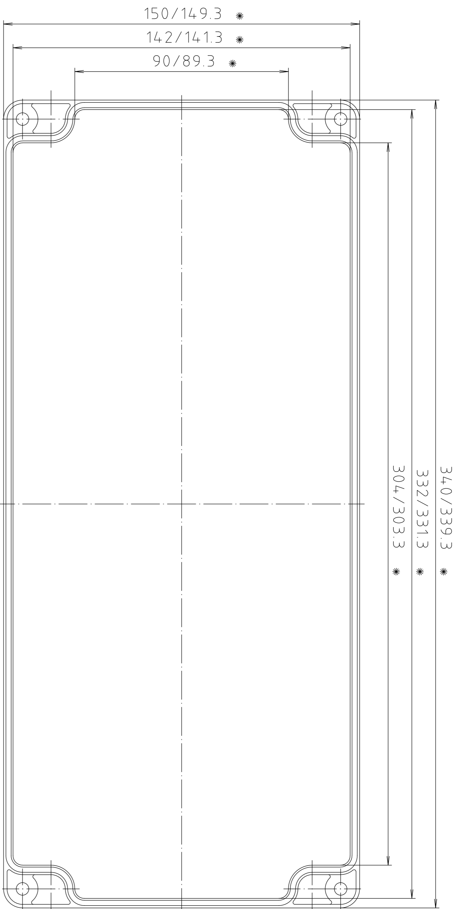
Deckel/lid
